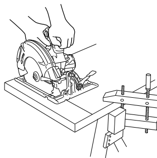
A TYPICAL ILLUSTRATION OF PROPER HAND SUPPORT WORKPIECE SUPPORT, AND SUPPLY CORD ROUTING.
